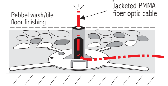
Installation profile
